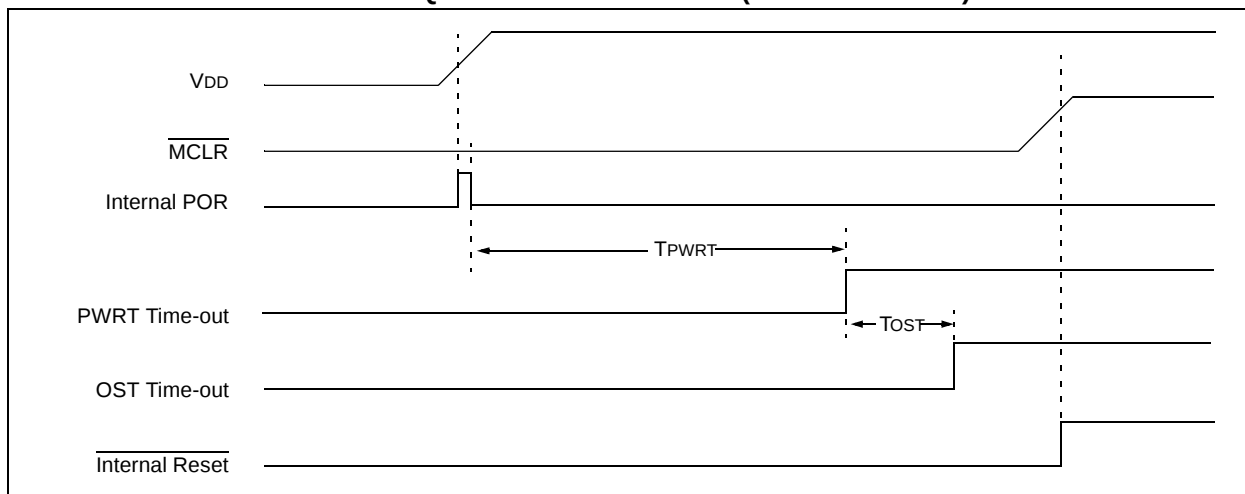
FIGURE 15-4: TIME-OUT SEQUENCE ON POWER-UP (DELAYED \overline{\text{MCLR}} ): CASE 2
