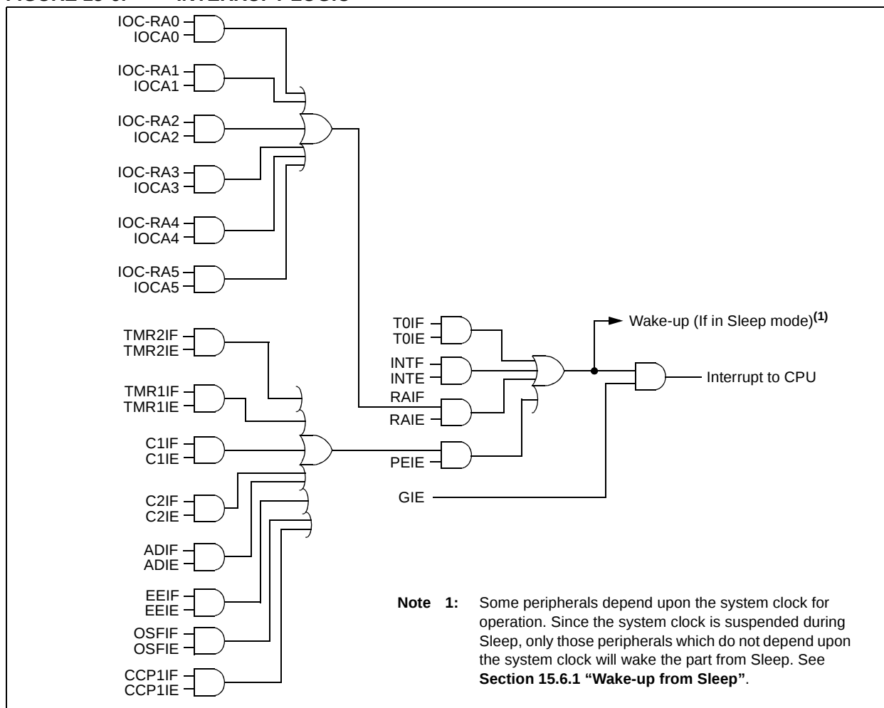
FIGURE 15-6: INTERRUPT LOGIC
