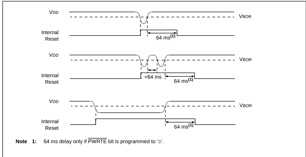
FIGURE 15-2: BROWN-OUT SITUATIONS
