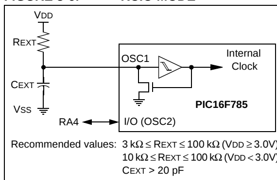
FIGURE 3-6: RCIO MODE
