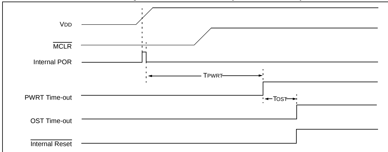
FIGURE 15-3: TIME-OUT SEQUENCE ON POWER-UP (DELAYED \overline{\text{MCLR}} ): CASE 1
