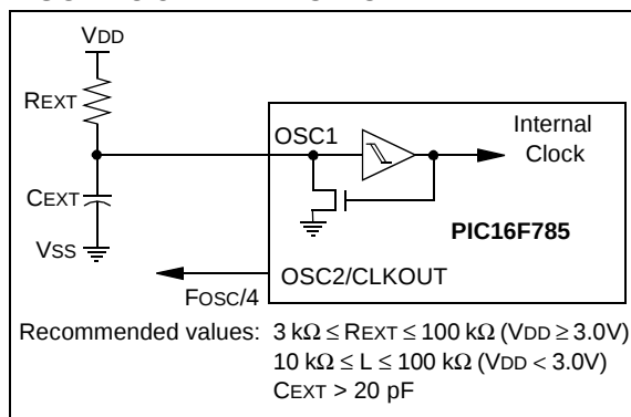
FIGURE 3-5: RC MODE
